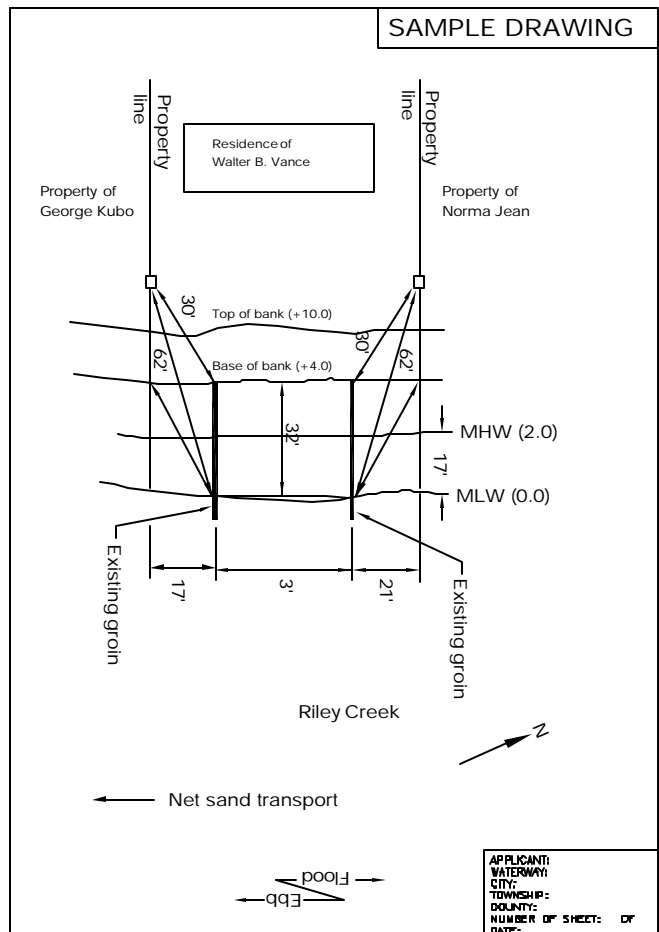
Beach Nourishment
